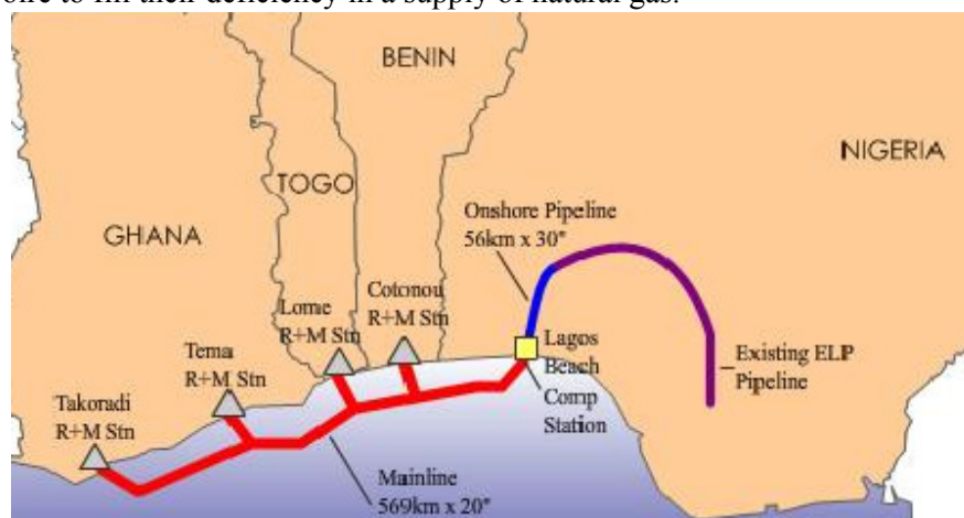
Figure 7.2.19 Route of West Africa Gas Pipeline (WAGP)
