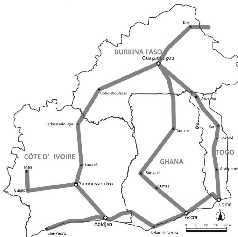
Figure 7.2.16 Major Optic Fibre Network in WGRIC Sub-Region
