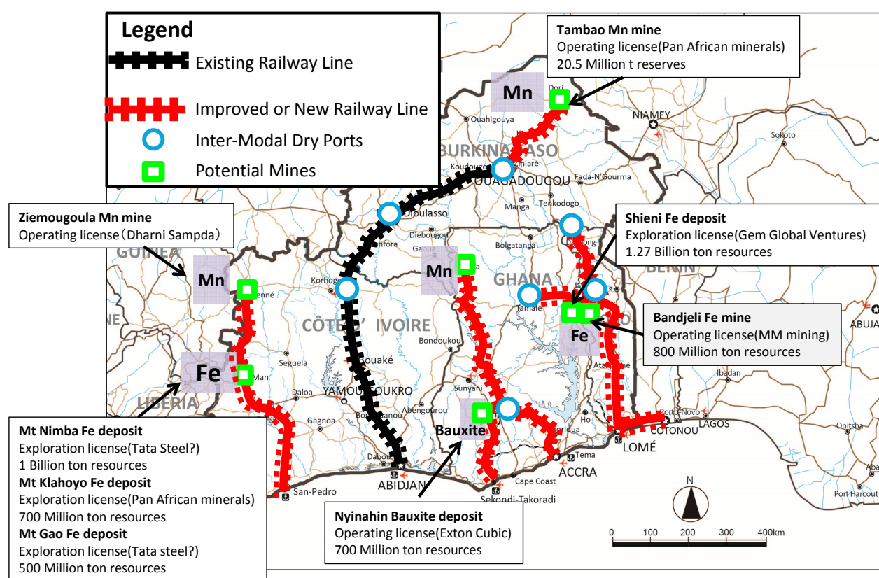
Figure 7.2.7 Bulk Mineral Resources and Railway Development
