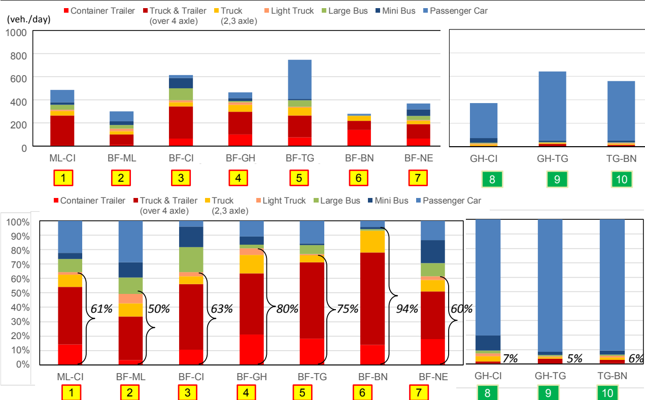
Figure 7.3.12 Daily Traffic Volume on Arterial Roads in WAGRIC Countries
