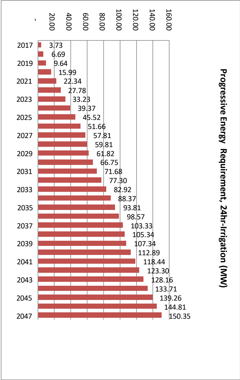
Figure 14.18: Progressive energy requirement for Irrigation (24hr)
