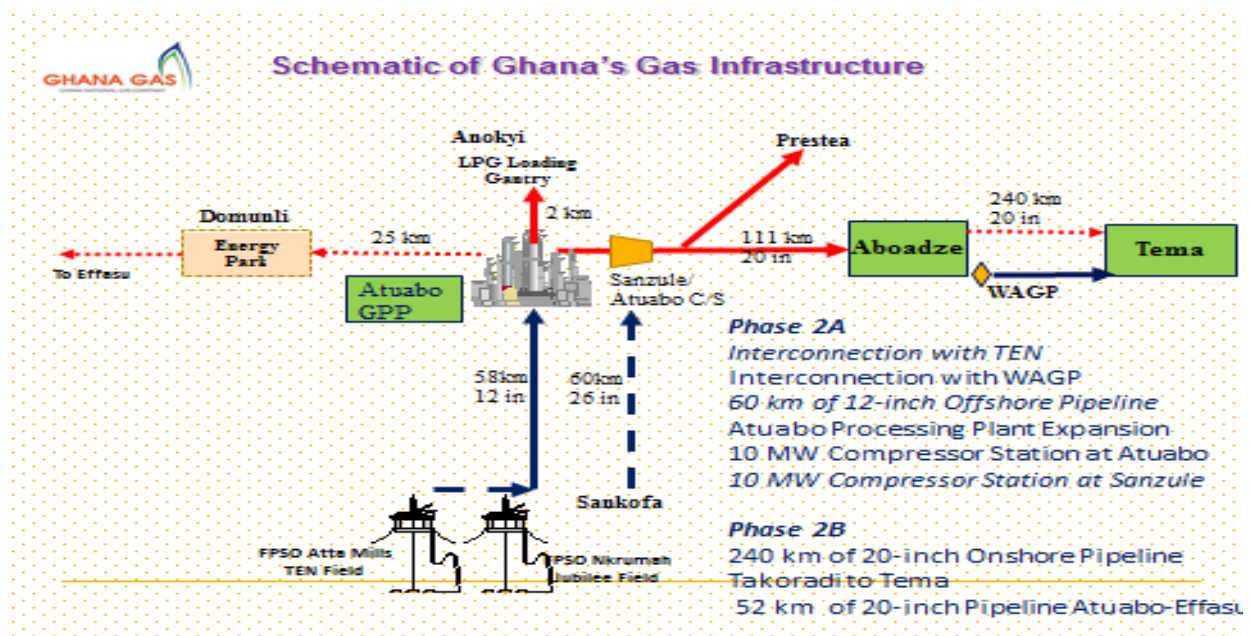
Figure 5.14: Ghana Gas Infrastructure Phase 2
