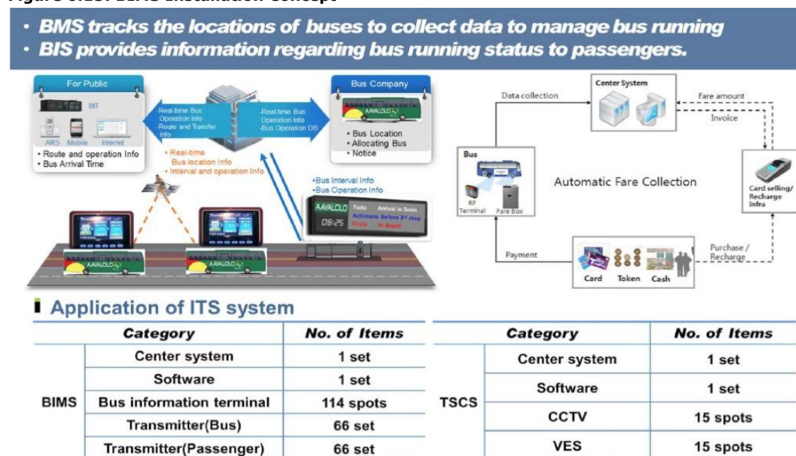
Figure 6.15: BIMS Installation Concept
